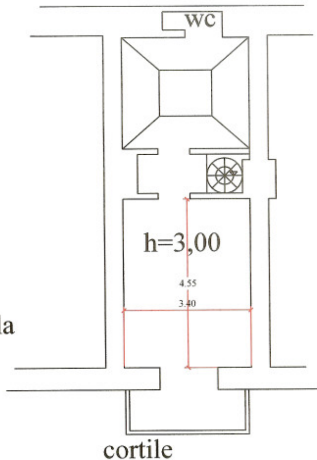
PIANO SOPPALCO
