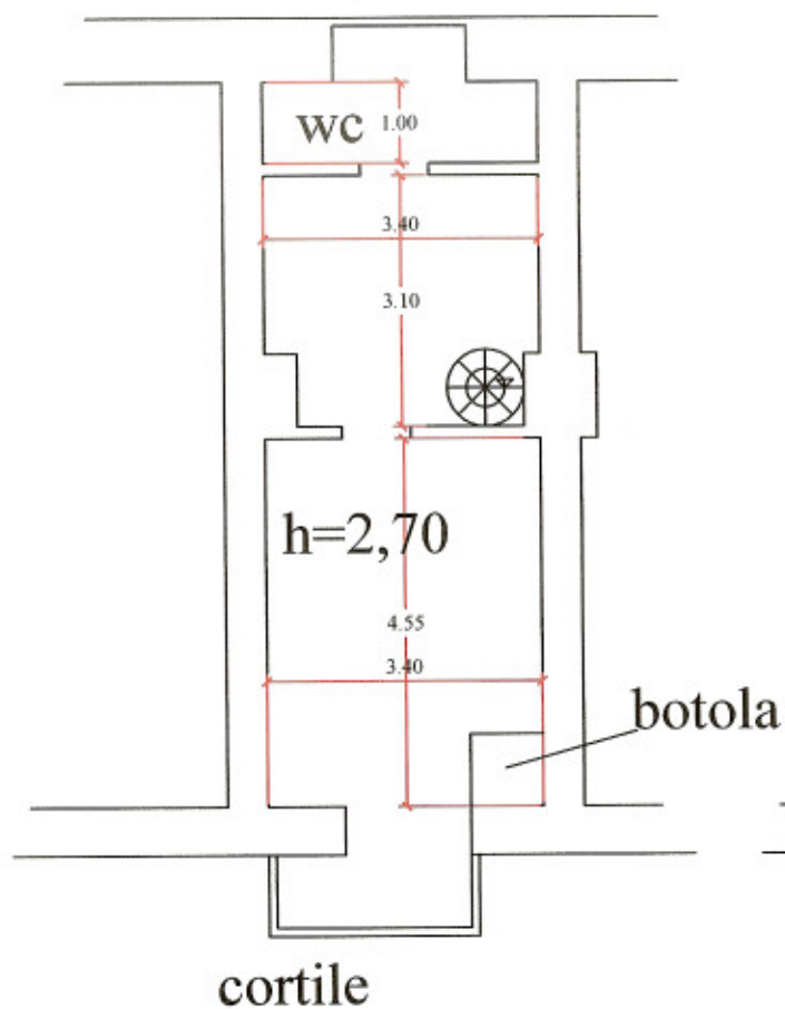
PIANO TERRA
